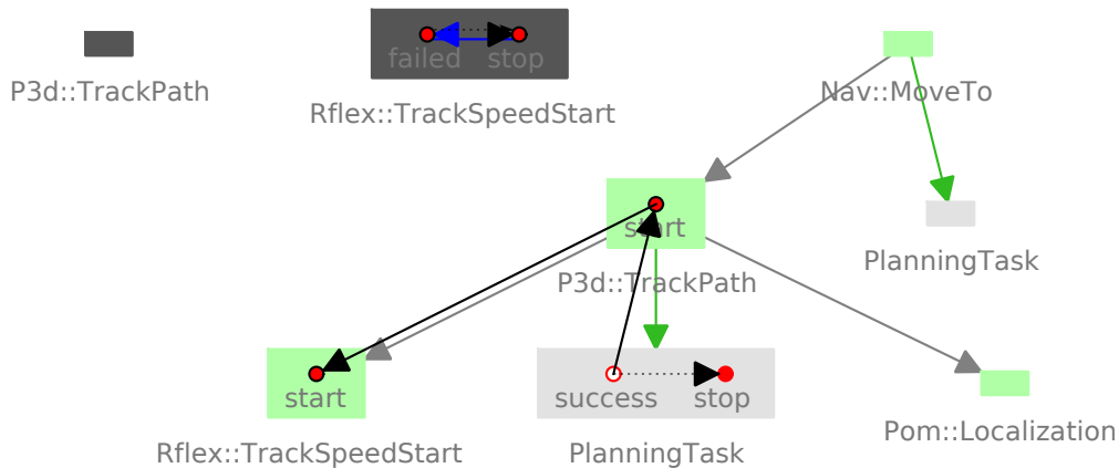
Figure 4.3: Result of the transaction on Fig. 4.2 when it is committed. The plan manager garbage-collected the old Rflex::TrackSpeedStart since it is not marked as useful anymore
