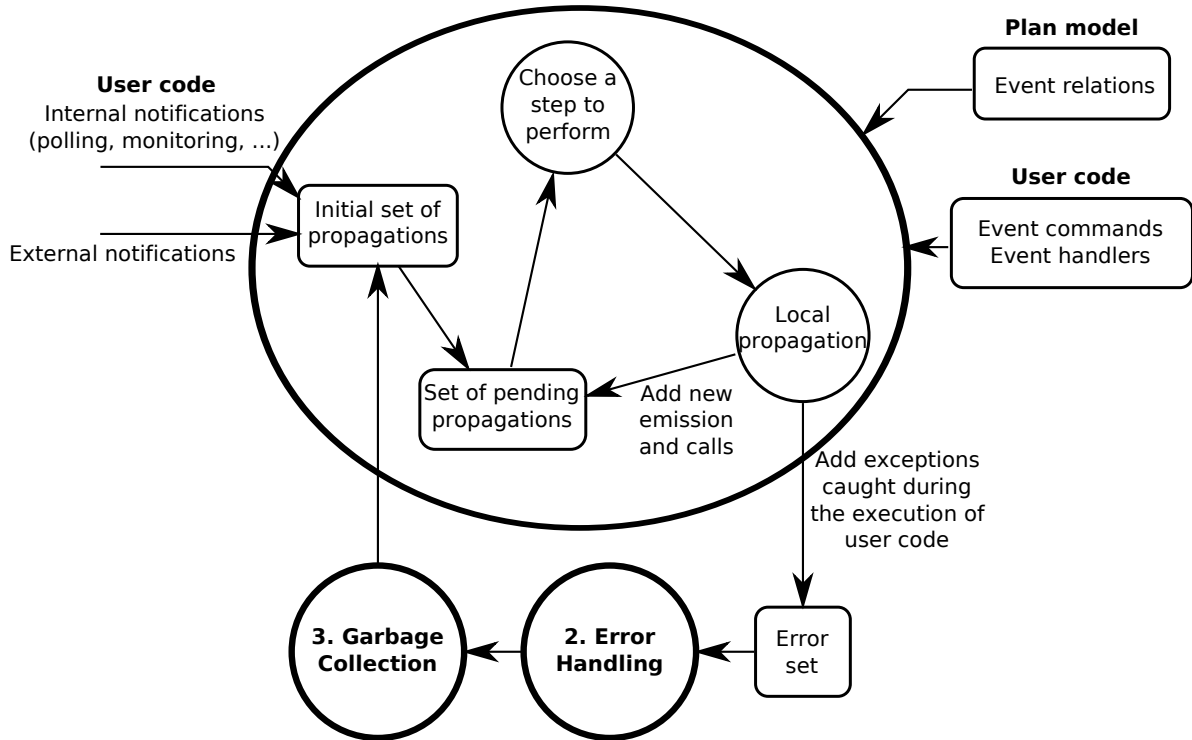
Figure 3.2: Overview of the event propagation phase: events are called or emitted by one by one, based on a set of pending operations, the plan and the user code.
