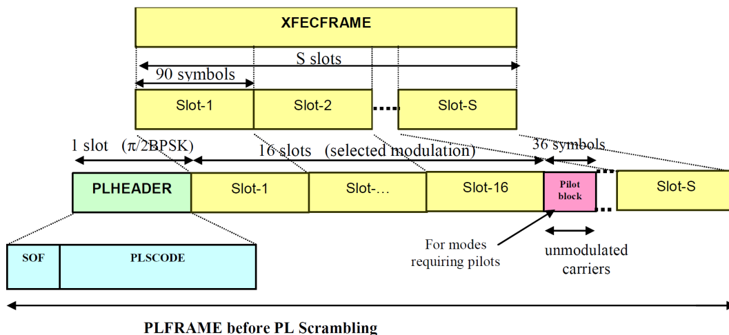
FIGURE 5.4 – Structure de PLFrame (DVB-RCS+M)
