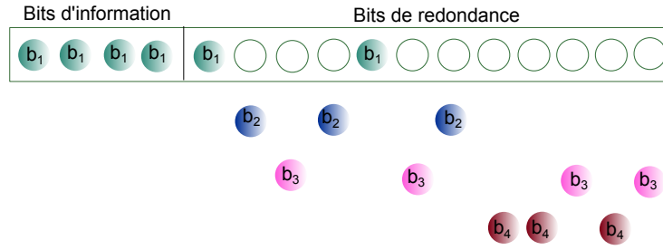
FIGURE 3.3 – Incremental redundancy HARQ
