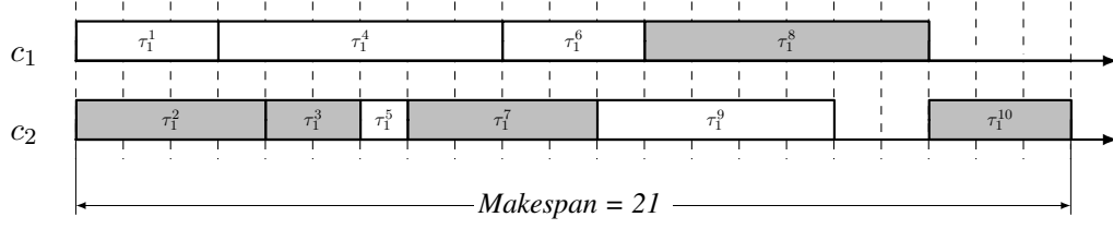
Figure 4.3: Example of schedule produced by HLFET on two cores. The sub-tasks of the critical path are colored in gray.
