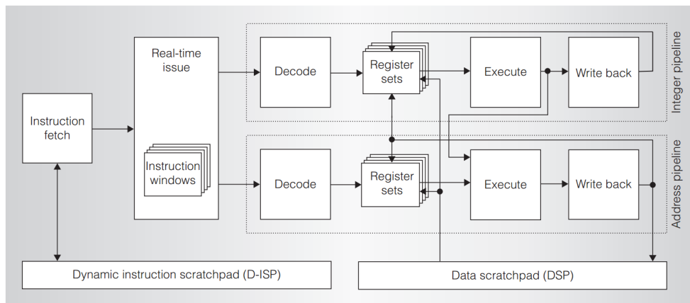
Figure 3.12: Block diagram of the Merasa architecture (extracted from [87]).
