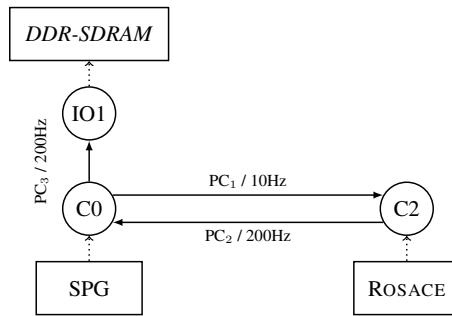
Figure 7.7: Budget of the ROSACE's partition with 2 PN and 3 PC
